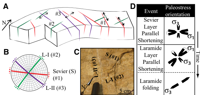
Figure 2. A: Sketch representing the vein network in the Bighorn Basin (Wyoming, USA). B: Orientation of the main vein sets encountered across the basin, corrected from strata tilting, reported on a lower hemisphere Schmidt stereonet; color code matches A. C: Field photograph illustrating chronological relationship of some fracture sets at Rattlesnake Mountain anticline (RMA). D: Successive orientations of horizontal principal stresses in the Bighorn Basin reconstructed from paleostress analyses (modified after Beaudoin et al., 2014).
