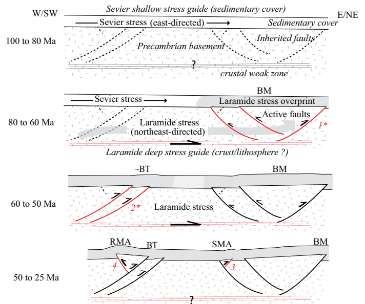
Figure 4. Evolution of thrust activation along a schematic W/SW-E/NE cross section of the Bighorn Basin (Wyoming, USA). Laramide stress overprint in the cover is reported as a gray shade. Activation of basement faults is symbolized by a red plane, and ages are inferred from published thermochronological data for the arch uplift and exhumation (noted *), and from U-Pb ages for the basin interior. BH—Bighorn Mountains; BT—Beartooth Mountains; RMA—Rattlesnake Mountain anticline; SMA—Sheep Mountain anticline.
